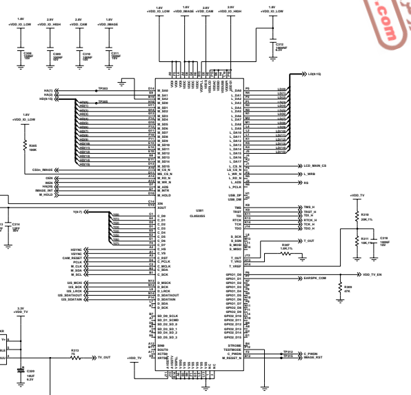
MULTIMEDIA CHIP (CL851S64)
